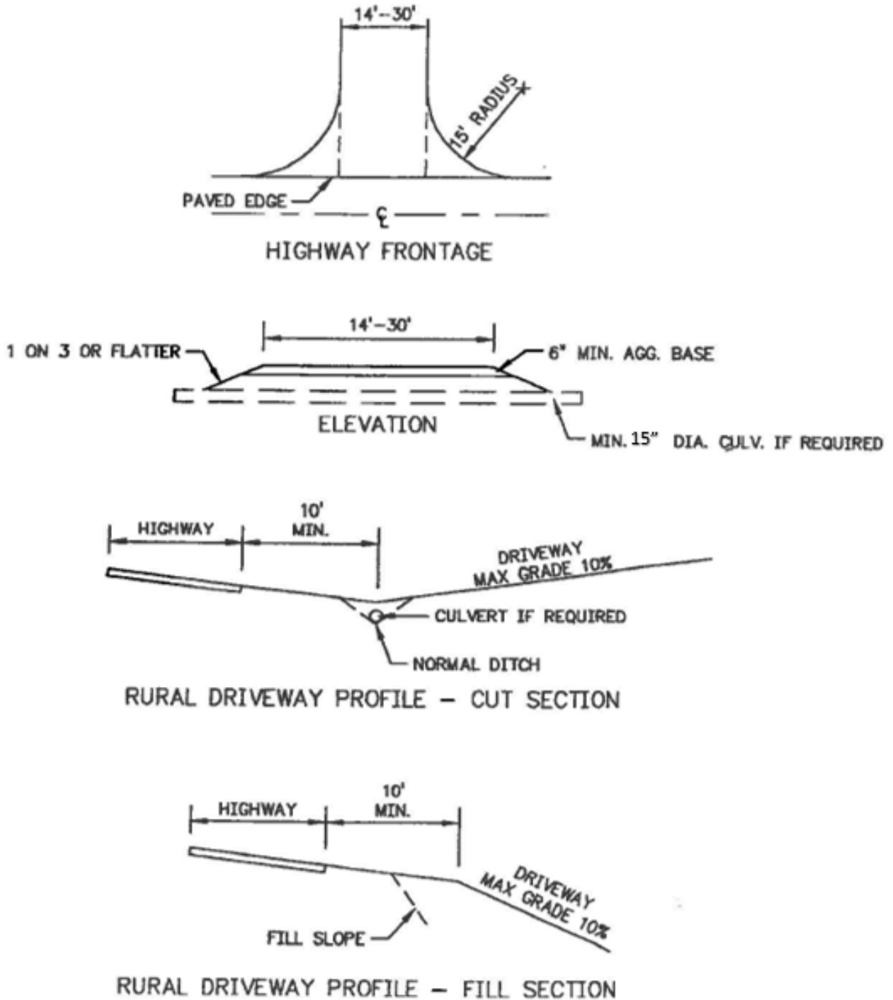
Figure 1 Drawing of driveway specifications
